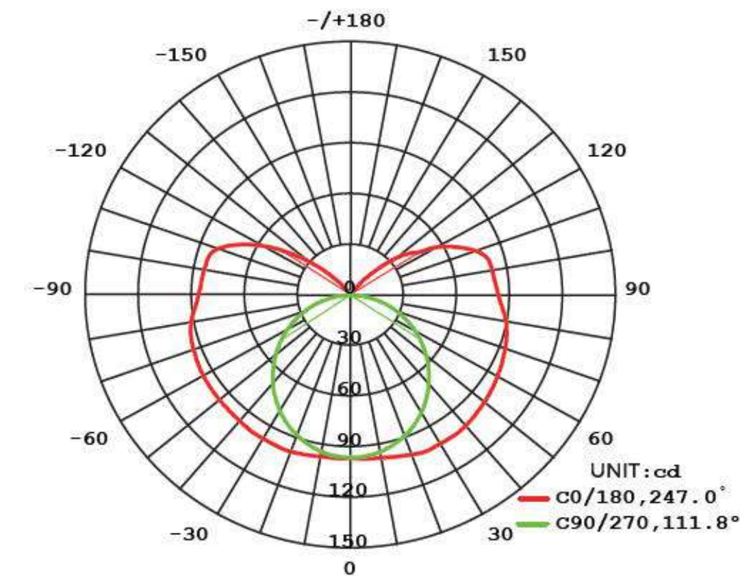
Light Distribution
