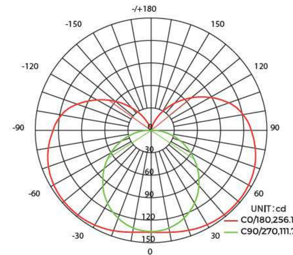
Light Distribution
