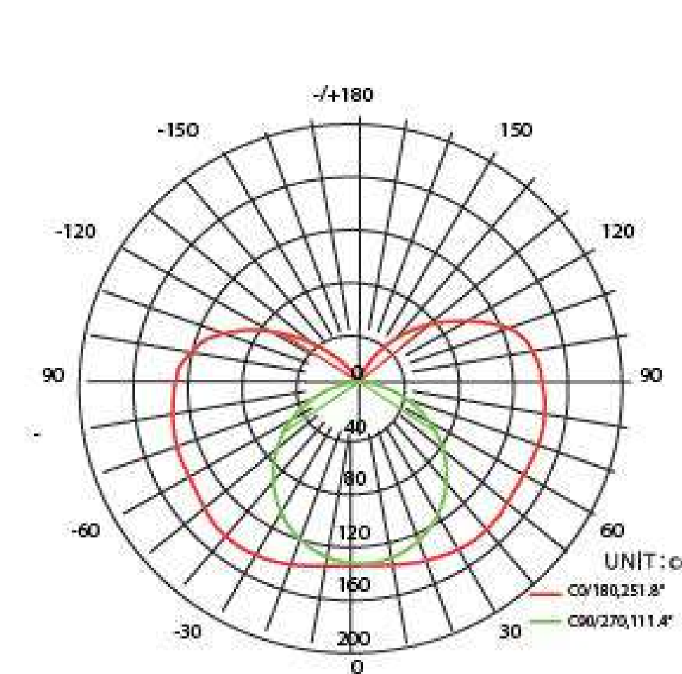
Light Distribution
