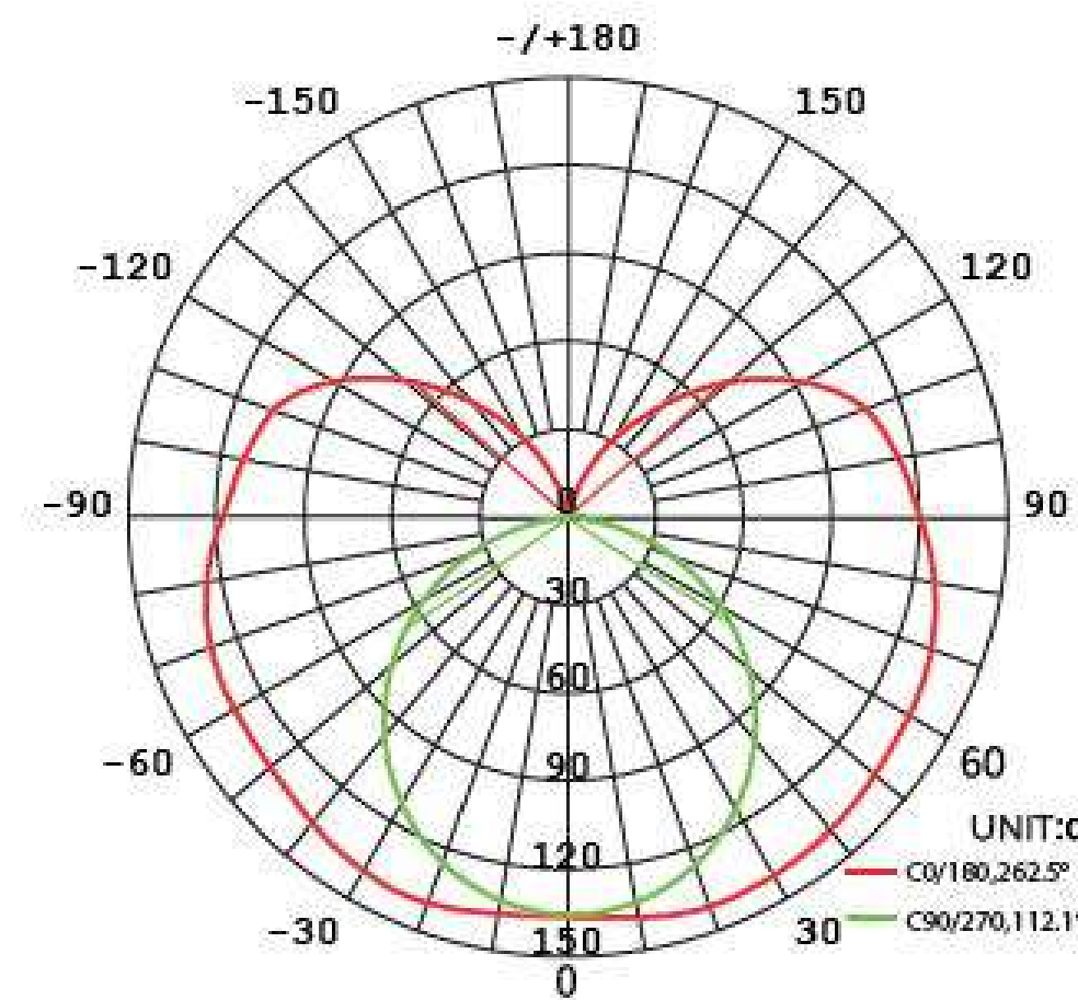
Light Distribution
